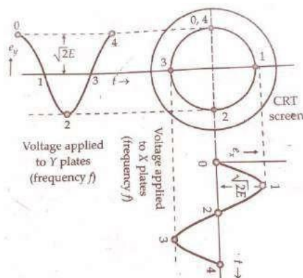
Figure: Lissajous figure for 90^\circ phase shift
