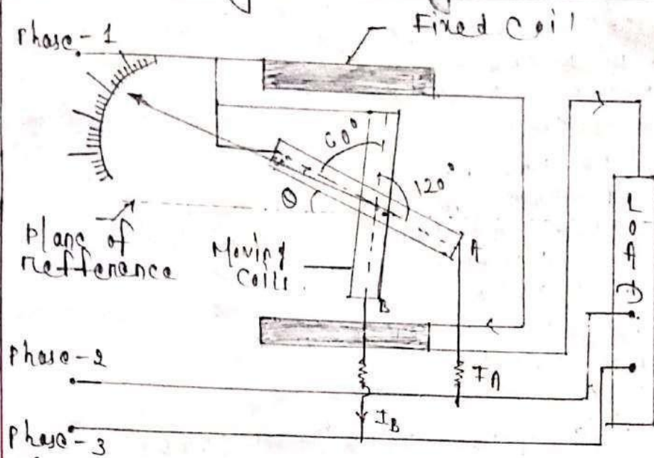
(Fig: 3-d Electrodynamometer type power factor meter)
