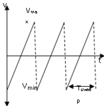
Figure: Sawtooth Waveform
